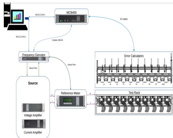
Figure 6. Schematic Diagram of Test setup in Laboratory
